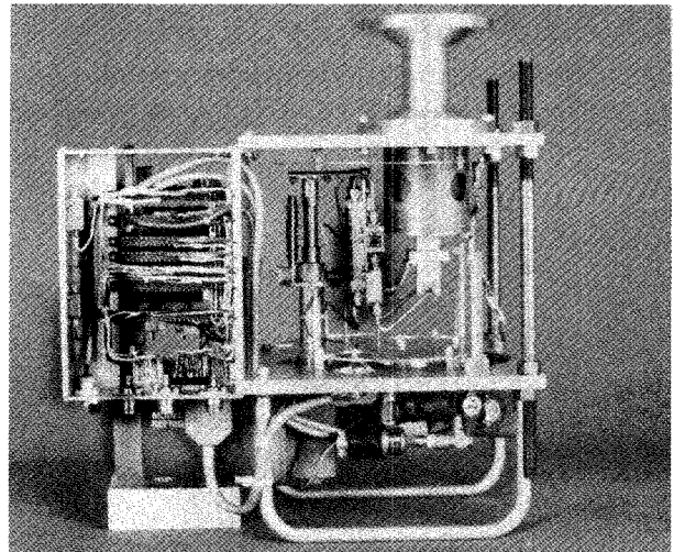
Fig. 5. Interior view of 8.4 GHz receiver. The vacuum cylindrical jacket and a radiation shield have been removed. From left to right the major components are a 300 K card cage for bias, control, monitor, and post amplifiers, the refrigerator cooling-head, amplifier mounting plate, and polarizer for both senses of circular polarization.
