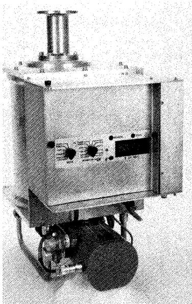
Fig. 4. Photograph of 4.8 GHz VLBA front-end. A typical front-end is ~ 30 cm wide and weighs 55 pounds. The input dual-polarization circular waveguide is shown at top. The front-end can be controlled and monitored either locally or by a remote computer.
