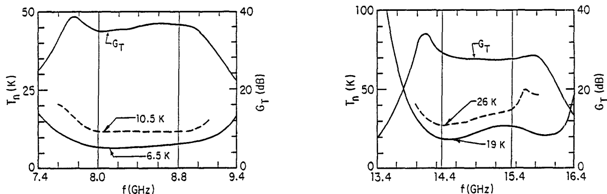
Fig. 2. Gain and noise temperature of HEMT amplifiers cooled to 15 K (solid lines) and total receiver noise (dashed lines) for both 8.4 GHz (left) and 14.9 GHz (right) receivers. The amplifier noise is referred to the cooled amplifier input connector while the receiver noise is referred to a 300 K waveguide flange.
