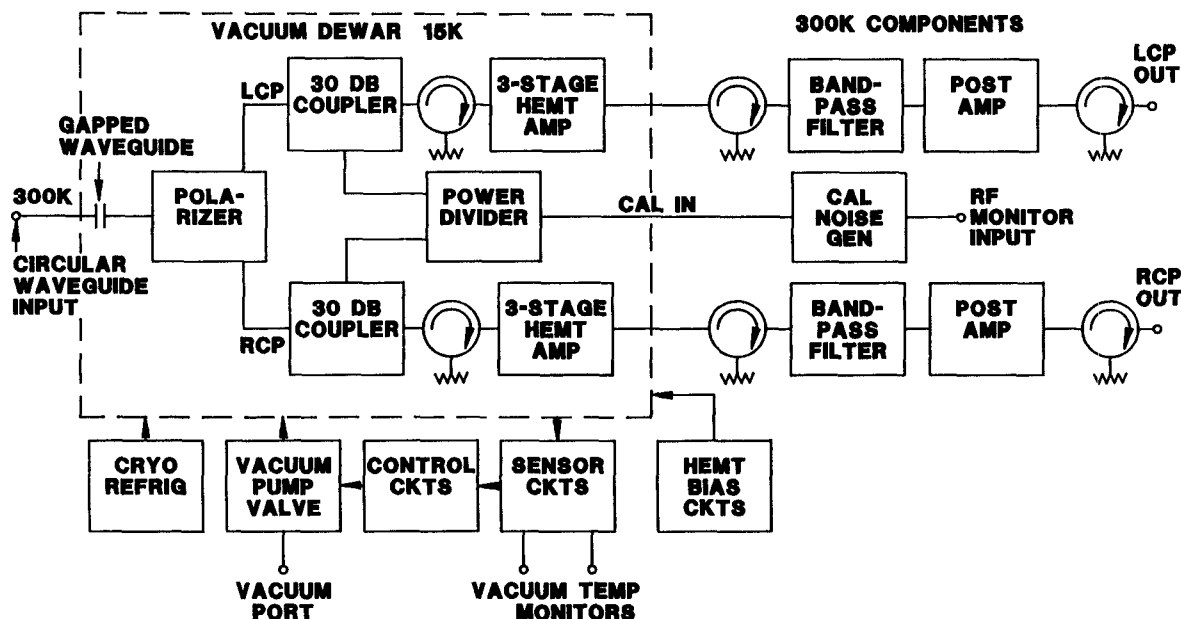
Fig. 3. Block diagram of typical VLBA front-end. For 8.4 GHz and above, the polarizer is cooled to 15 K rather than 50 K. Also, for frequencies above 4.6 GHz, isolators are placed at amplifier inputs. Approximately 30 dB gain at 15 K and 20 dB gain at 297 K is provided.
