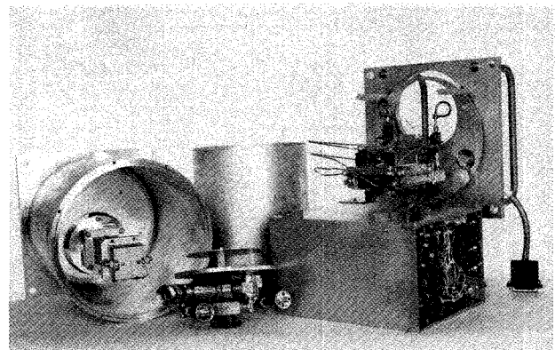
Fig. 6. A partially disassembled view of the 8.4 GHz receiver. From left to right the components are the cylindrical vacuum jacket with polarizer mounted to top plate, (foreground) an access cover with vacuum valves and gauge, (background) a 50 K radiation shield, and the card cage with amplifier mounting plate (refrigerator removed).
